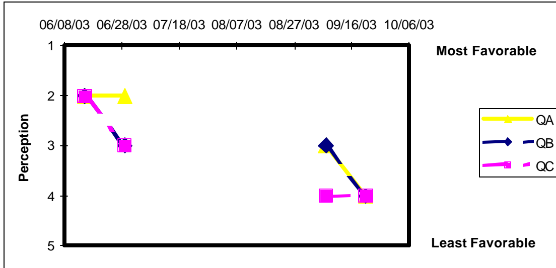
Figure 27. 2003 Lake Perception Data for Findley Lake
