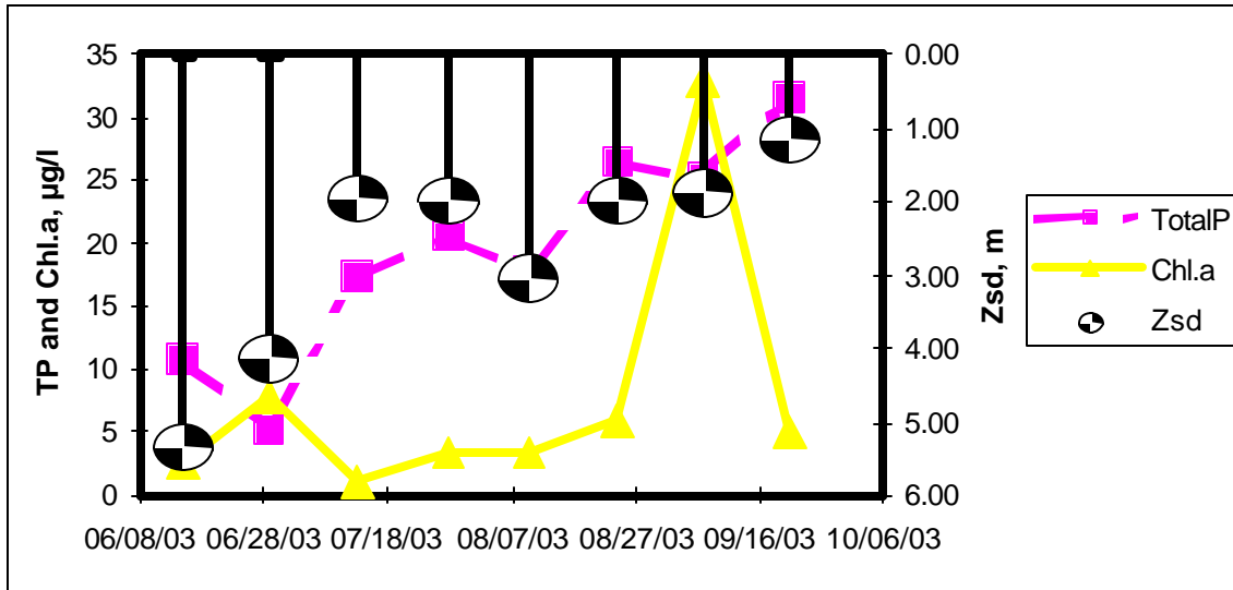
Figure 15. 2003 Eutrophication Data for Findley Lake
