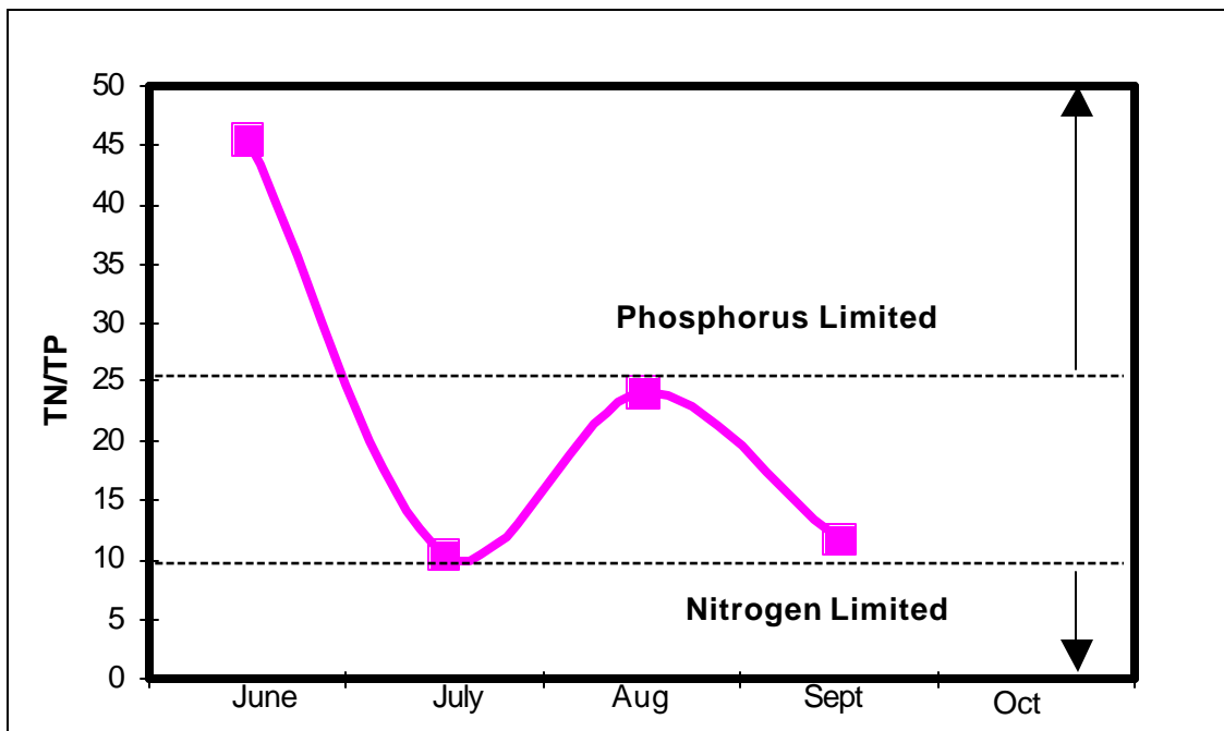
Figure 18- Nitrogen to Phosphorus Ratios in a Typical (Monthly Mean) Year for Findley Lake
