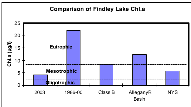
Figure 30. Comparison of 2003 Chlorophyll a to Lakes with the Same Water Quality Classification, Neighboring Lakes, and Other CSLAP Lakes in 2003
