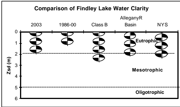
Figure 29. Comparison of 2003 Secchi Disk Transparency to Lakes With the Same Water Quality Classification, Neighboring Lakes, and Other CSLAP Lakes in 2003
